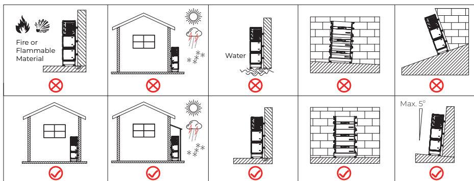
Figure 6-2 Installation Angle
