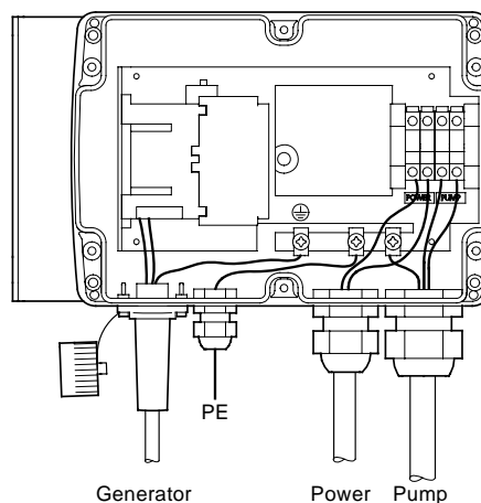
Fig. 23 Electrical connections
